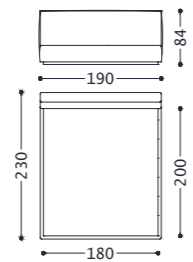
1DILLA180B 2DILLA180B
