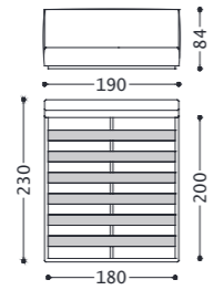
1DILLA180 2DILLA180
