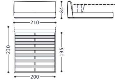
1DILLB200AF 2DILLB200AF
