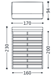
1DILLA160H 2DILLA160H
