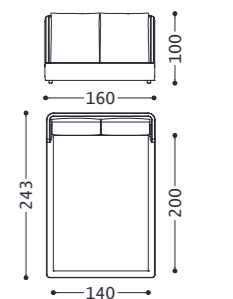
1NKLLA140B 2NKLLA140B
